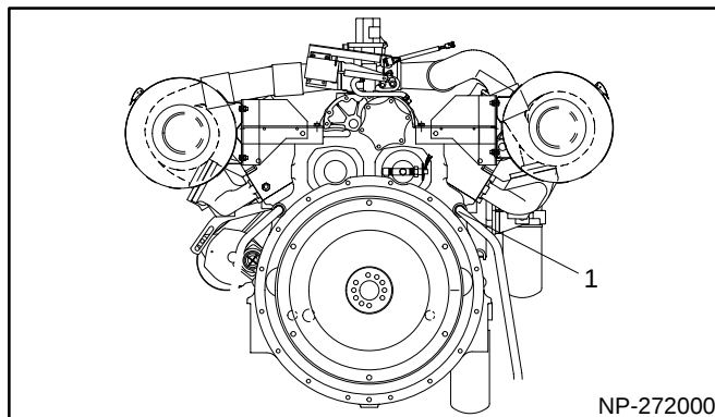
Figure 4. Engine—Rear View
