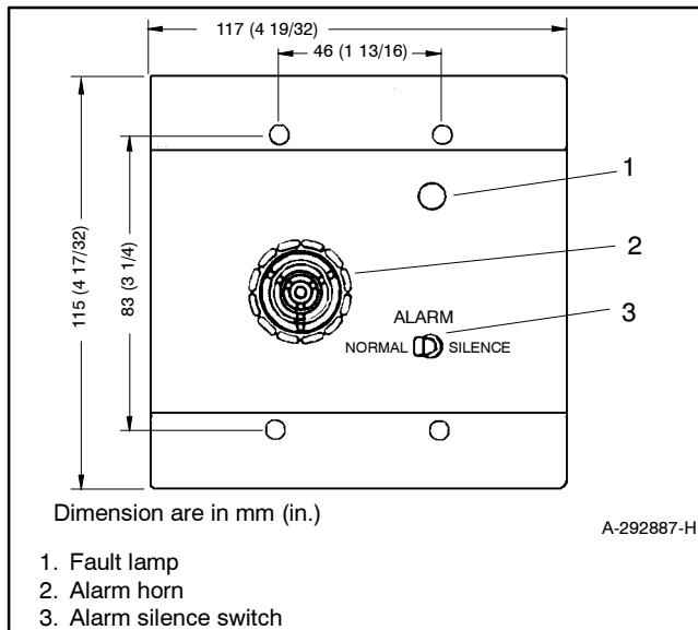
Figure 1 Audiovisual Alarm Panel
