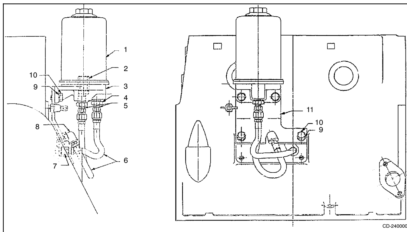
Figure 1 Oil Filter Kit
