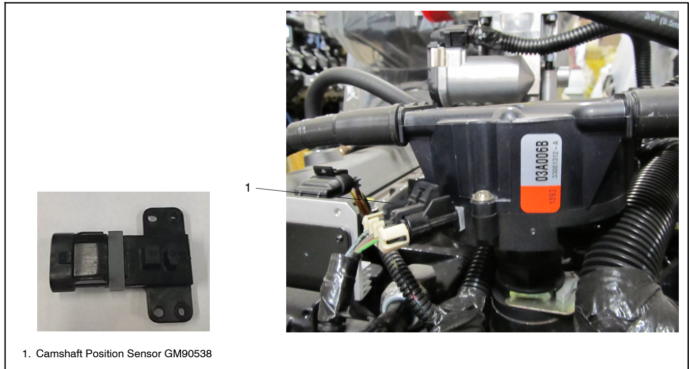
Figure 1 Camshaft Position Sensor
