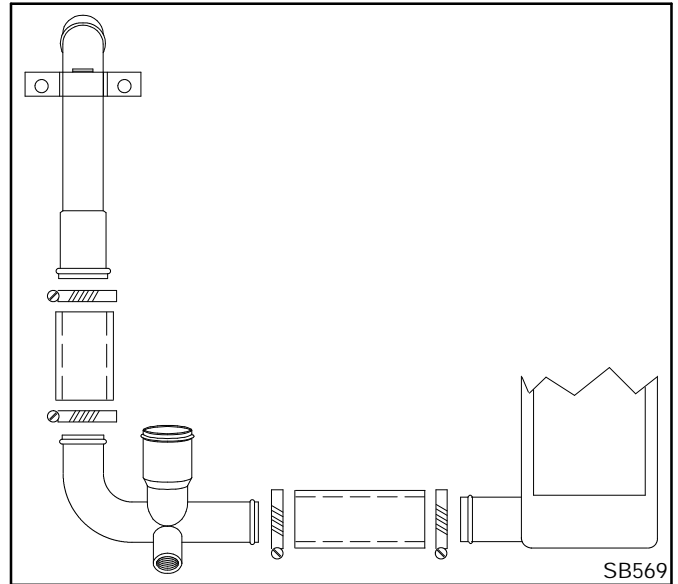
Figure 1. Radiator Outlet Tube Kit
