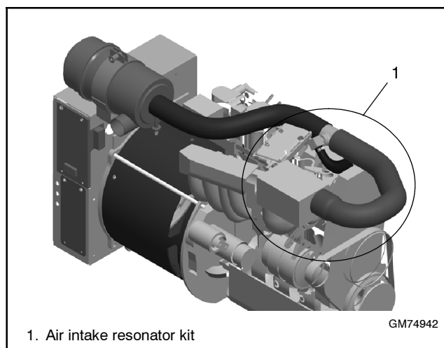
Figure 1 Air Intake Resonator Kit, Installed
