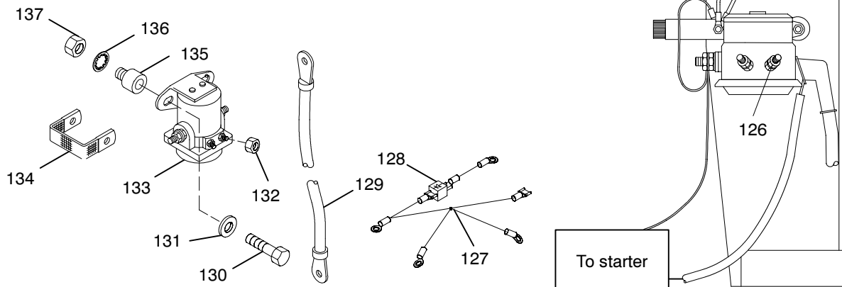
A Starter Solenoid
