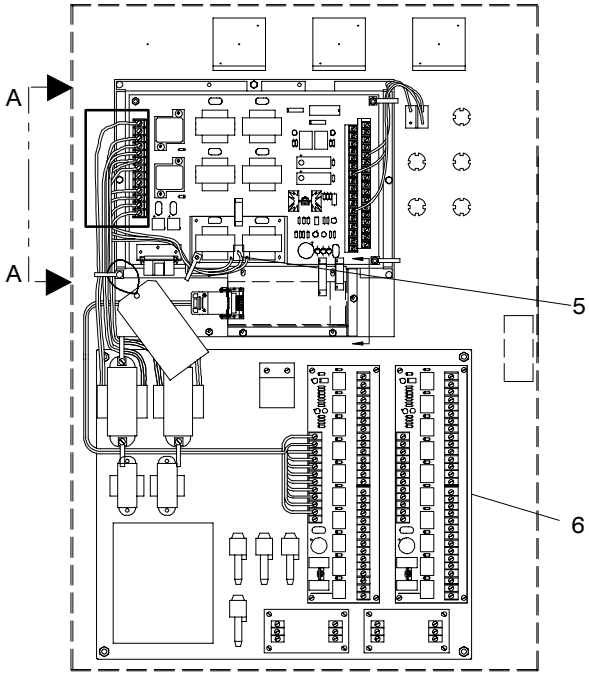
Barrier Assembly
