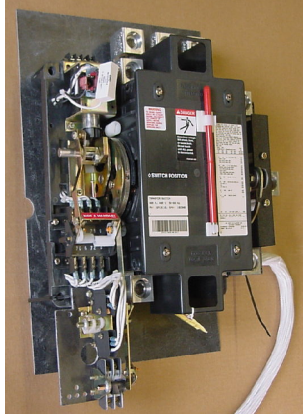
Model KCT 225, 230 (600 V), 260, 400 Amp
