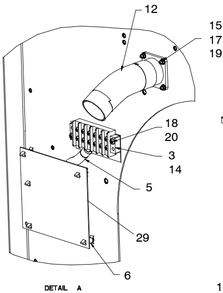
Non-DEC 550 Controller
