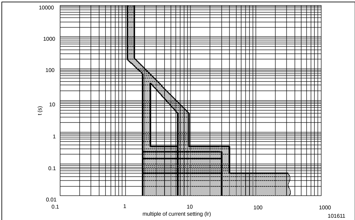
Figure 11. Time Current Curves, Circuit Breaker Style 1601
