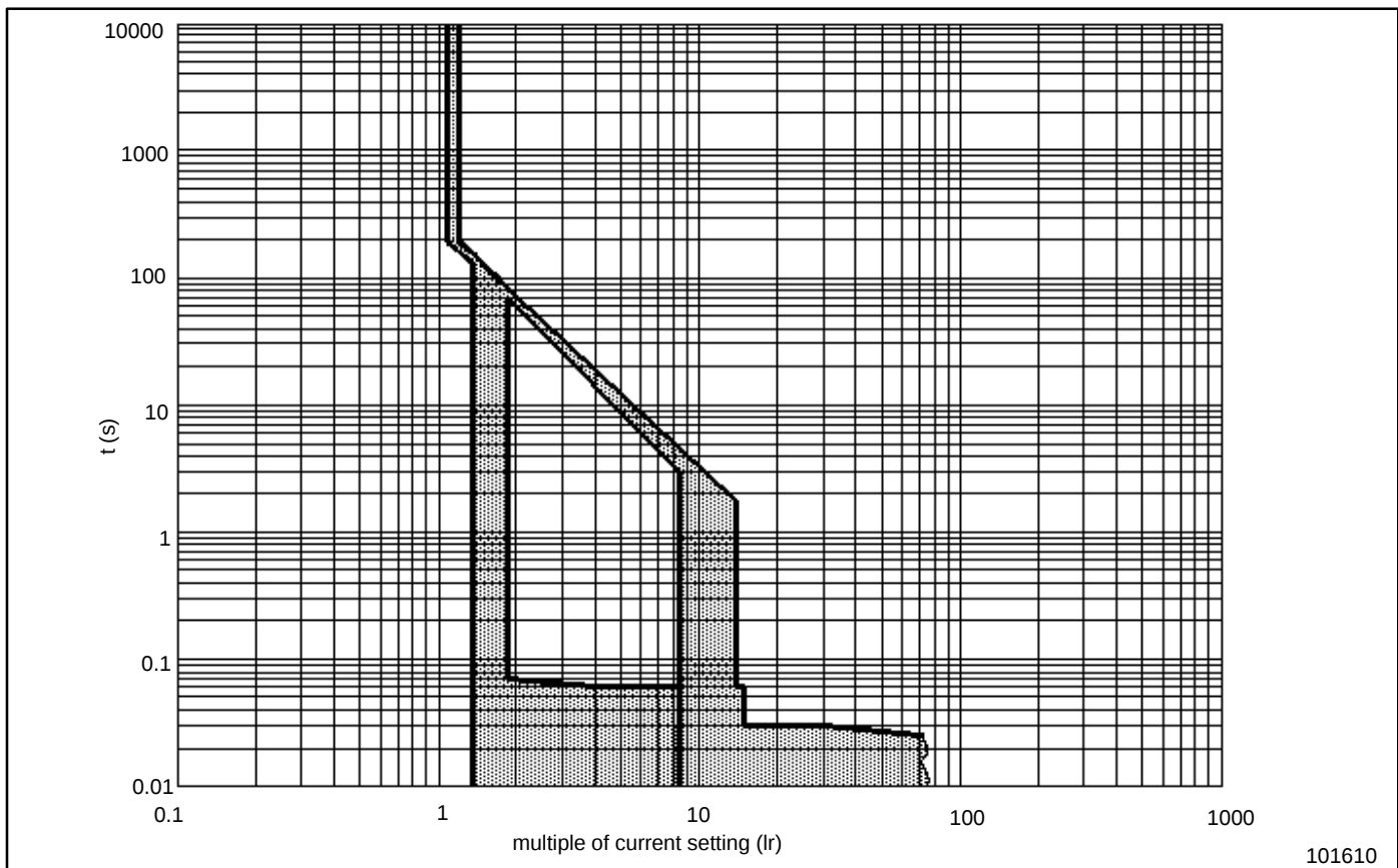
Figure 10. Time Current Curves, Circuit Breaker Style 1600
