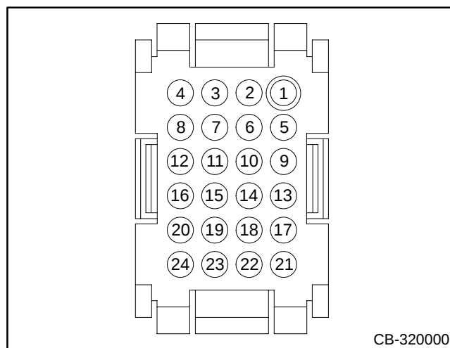
Figure 3. Plug P1
