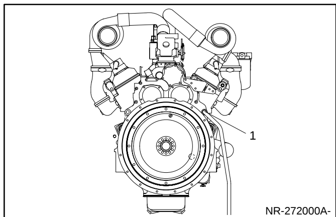
Figure 4. Engine—Rear View
