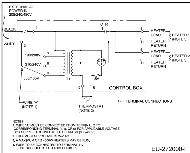
Figure 7. Terminal Connections for Block Heater Control Box
