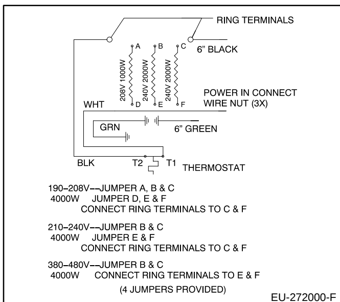
Figure 8. Block Heater Voltage Connections and Jumper Placement
