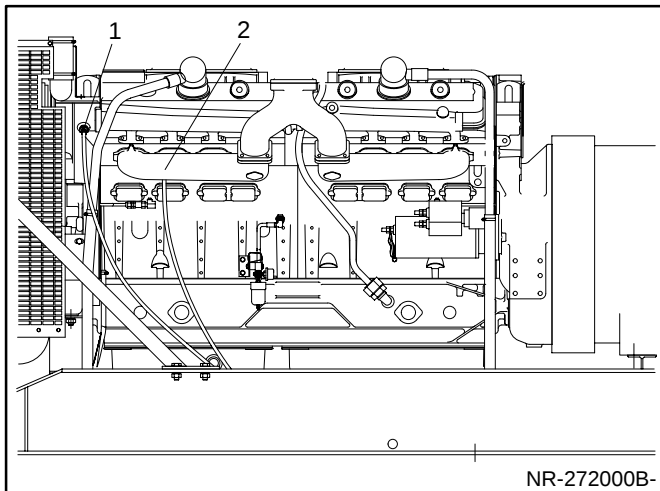
Figure 5. Engine—Left Side View
