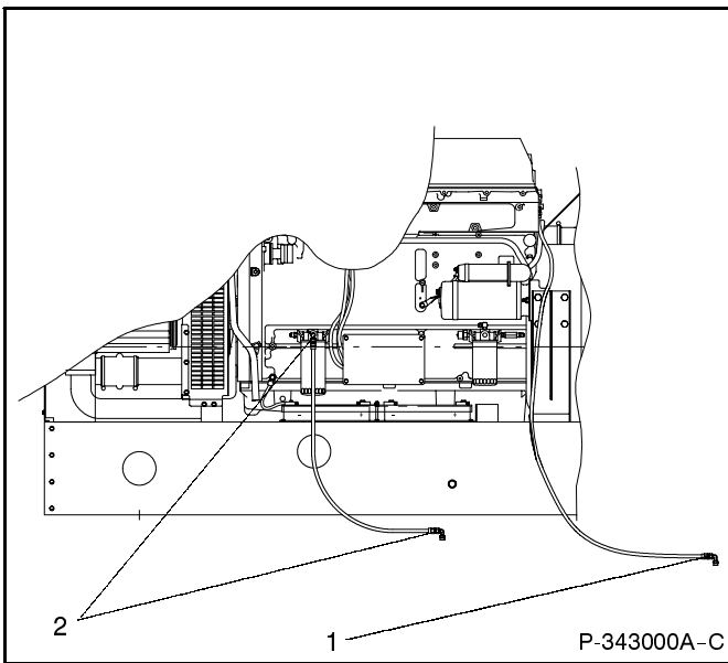
Figure 1. Oil Line Elbow and Flexible Fuel Line Locations
