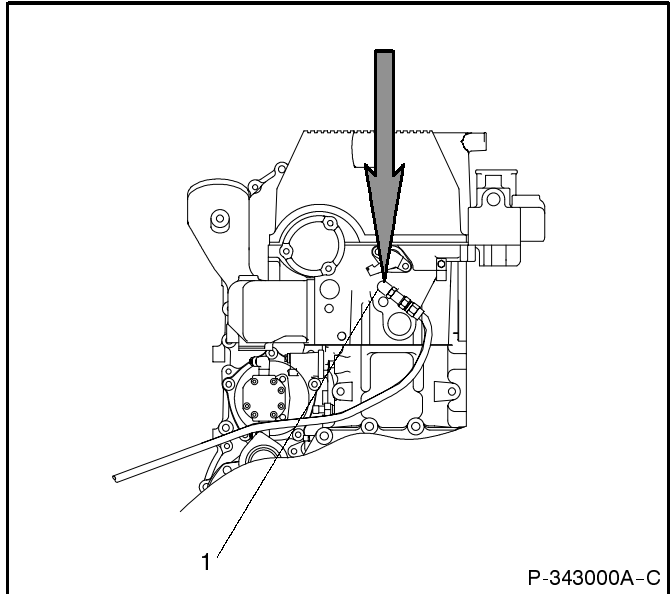
Figure 2. Oil Line Elbow Fitting Position
