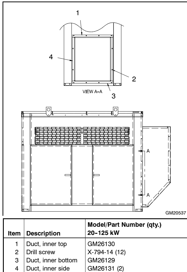
Figure 2 Installing Inner Duct Components
