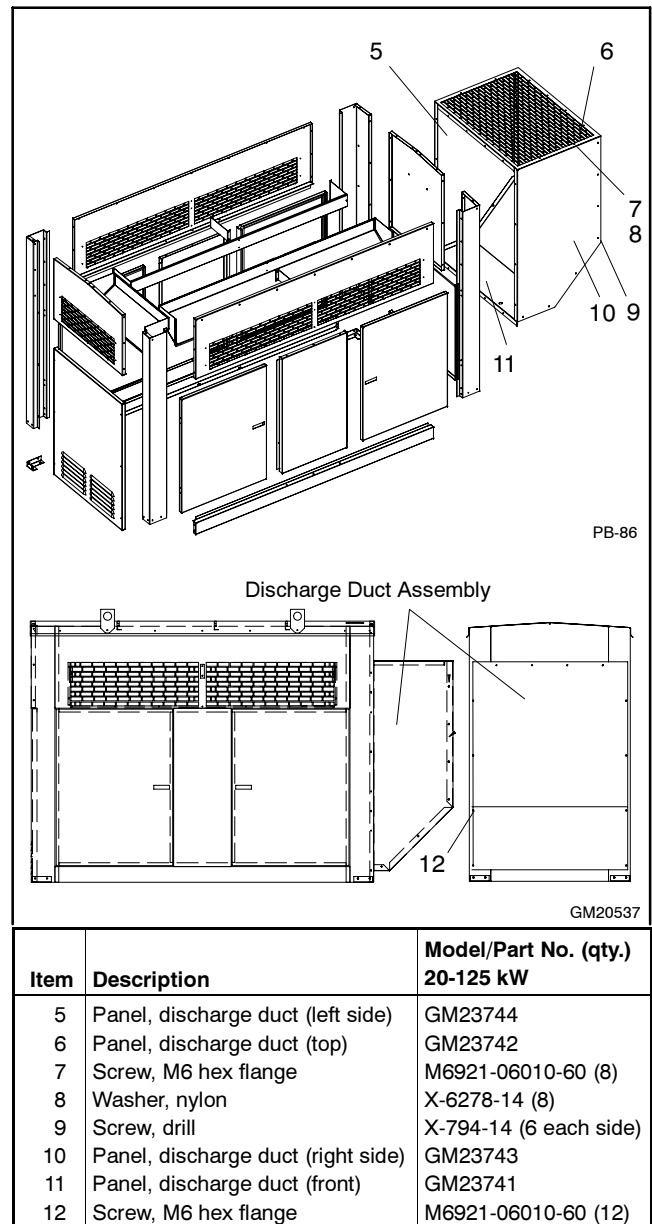
Figure 3 Assembling Discharge Duct
