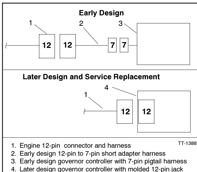
Figure 1 Governor Controller Configurations
