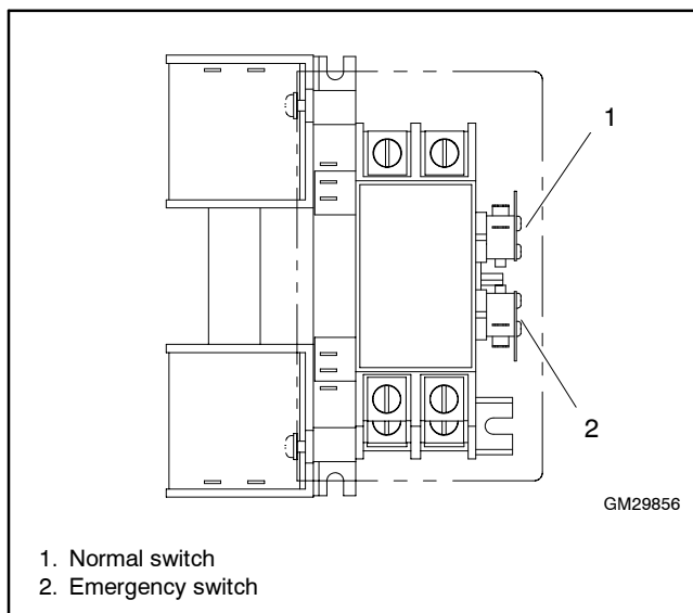
Figure 1 Auxiliary Switches
