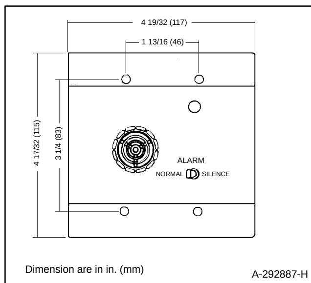
Figure 1. A/V Alarm Panel
