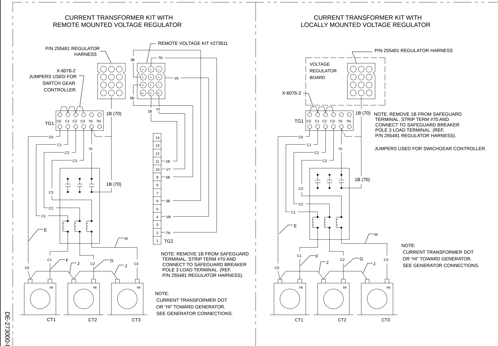
Figure 5. Current Transformer Circuit Connections
