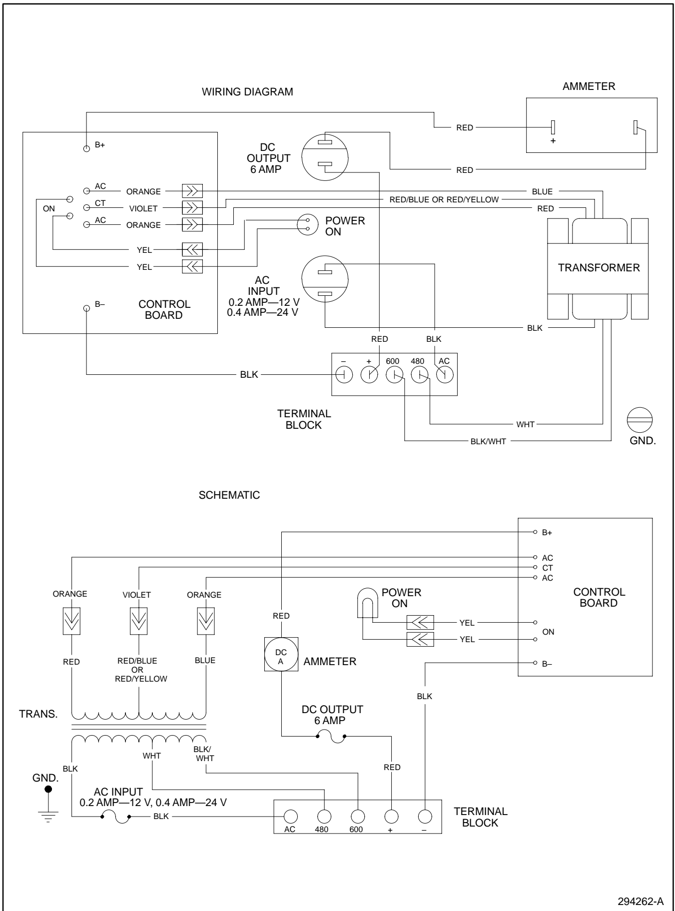
Figure 15. Wiring Diagram, Schematic—480/600-Volt Battery Charger
