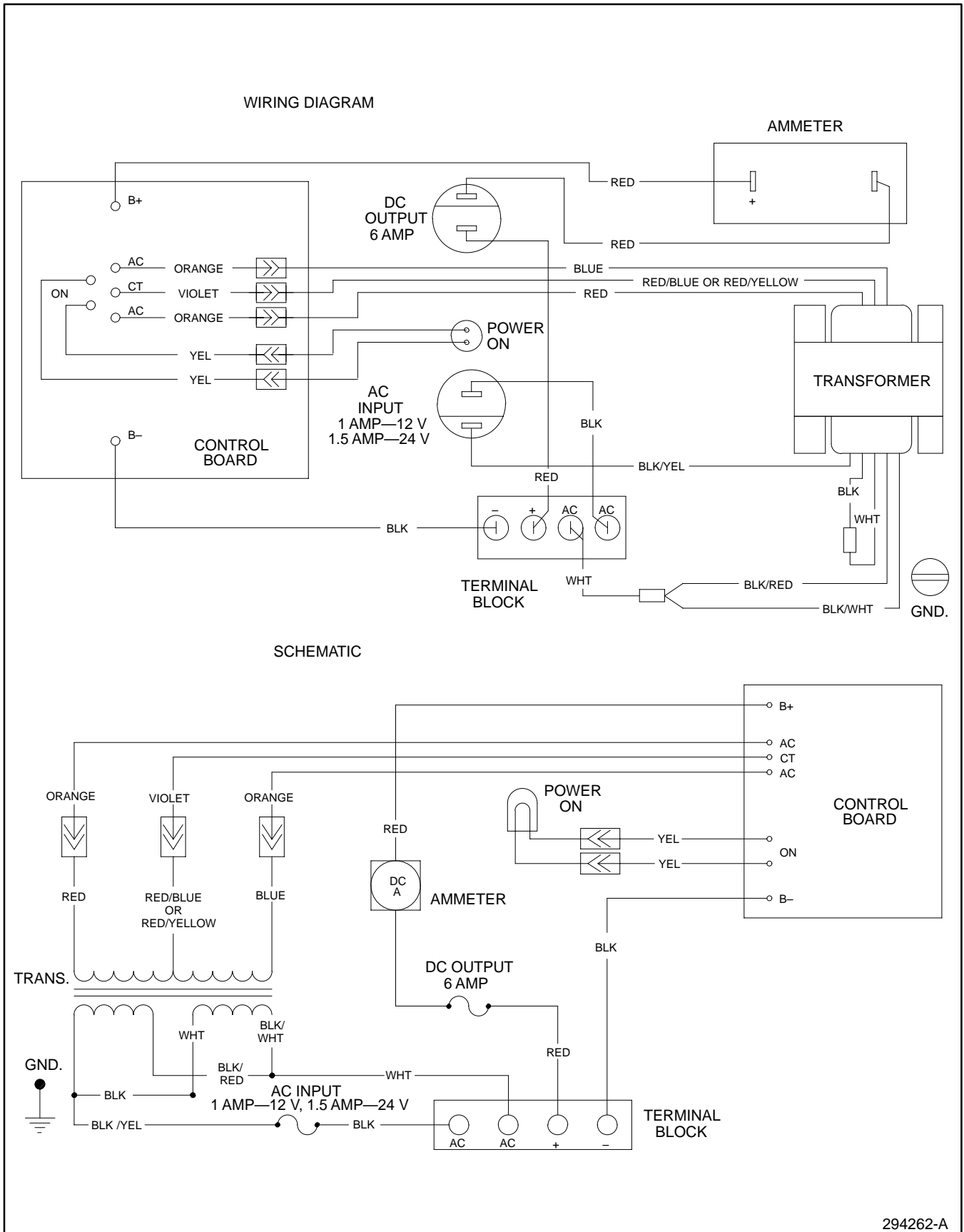
Figure 10. Wiring Diagram, Schematic—120-Volt Battery Charger
