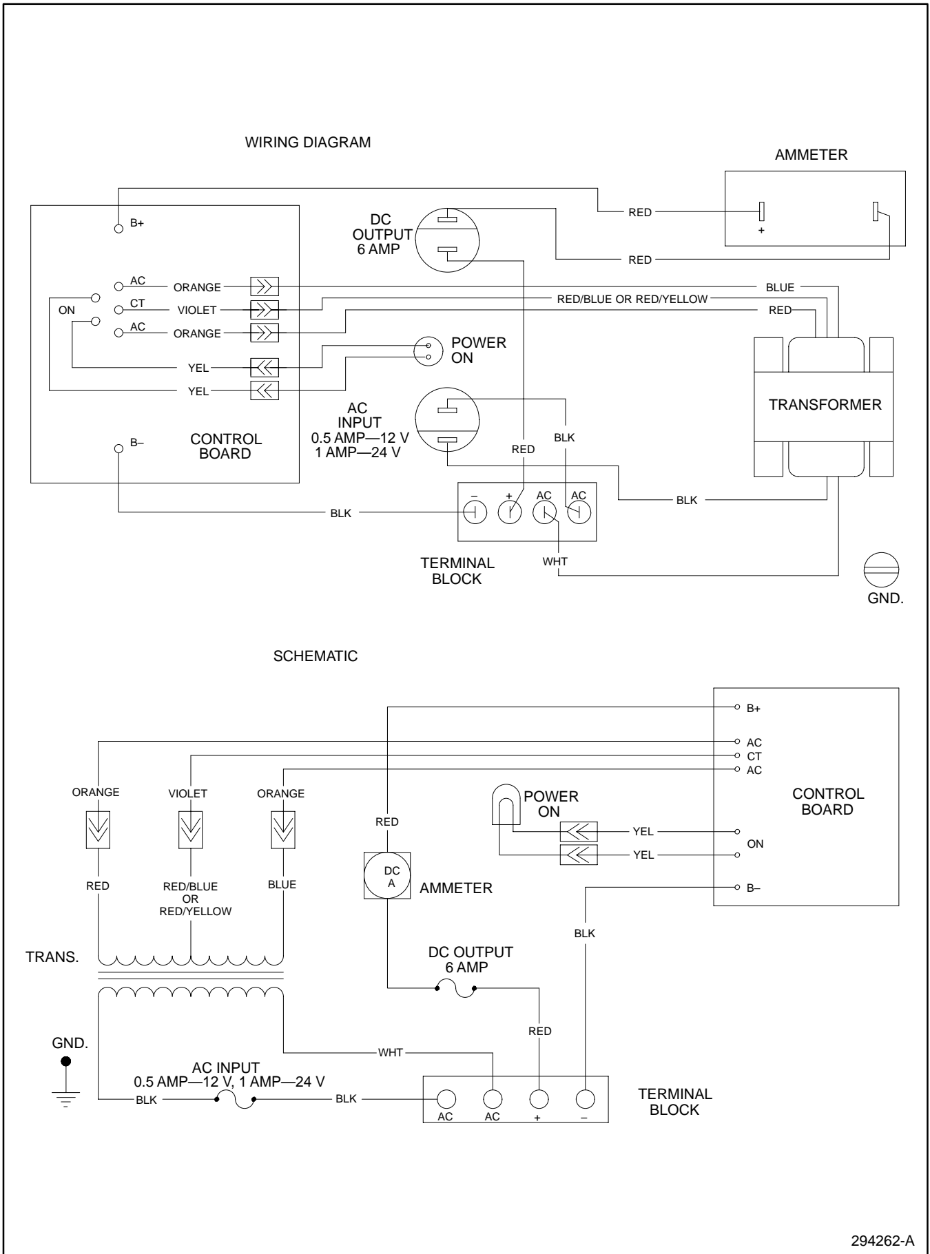
Figure 12. Wiring Diagram, Schematic—220-Volt Battery Charger
