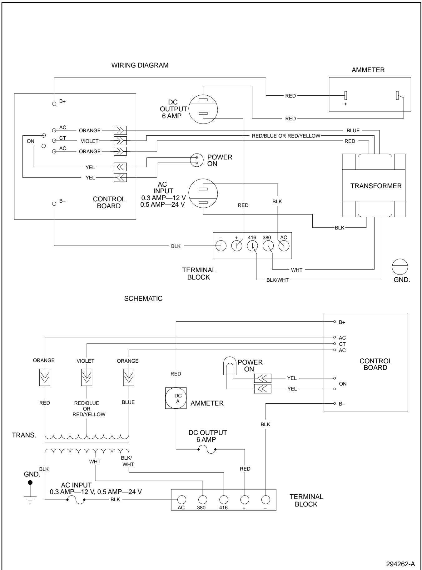
Figure 14. Wiring Diagram, Schematic—380/416-Volt Battery Charger
