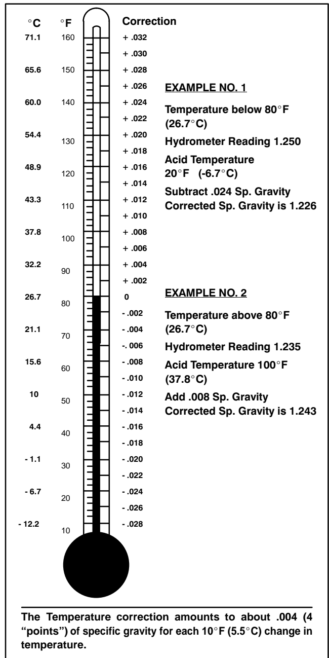
Figure 9. Specific Gravity Temperature Correction
