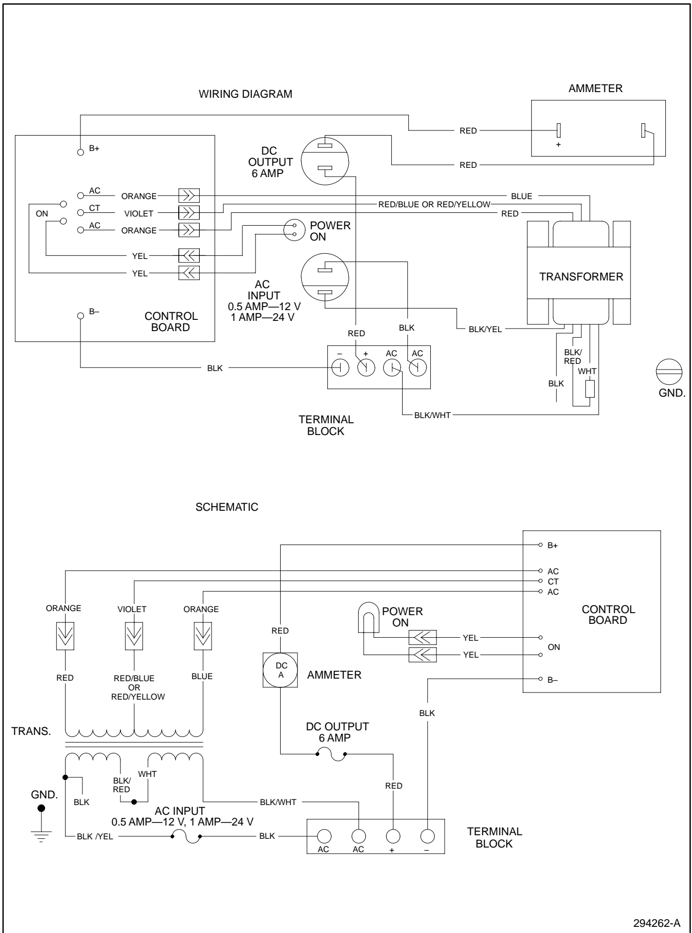
Figure 13. Wiring Diagram, Schematic—240-Volt Battery Charger
