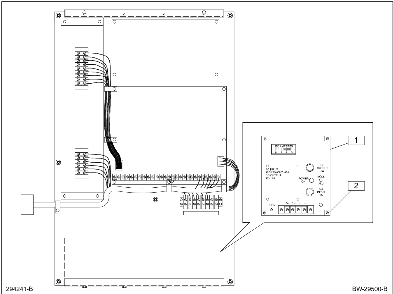
Figure 8. Battery Charger Installation—Solid-State Transfer Switch
