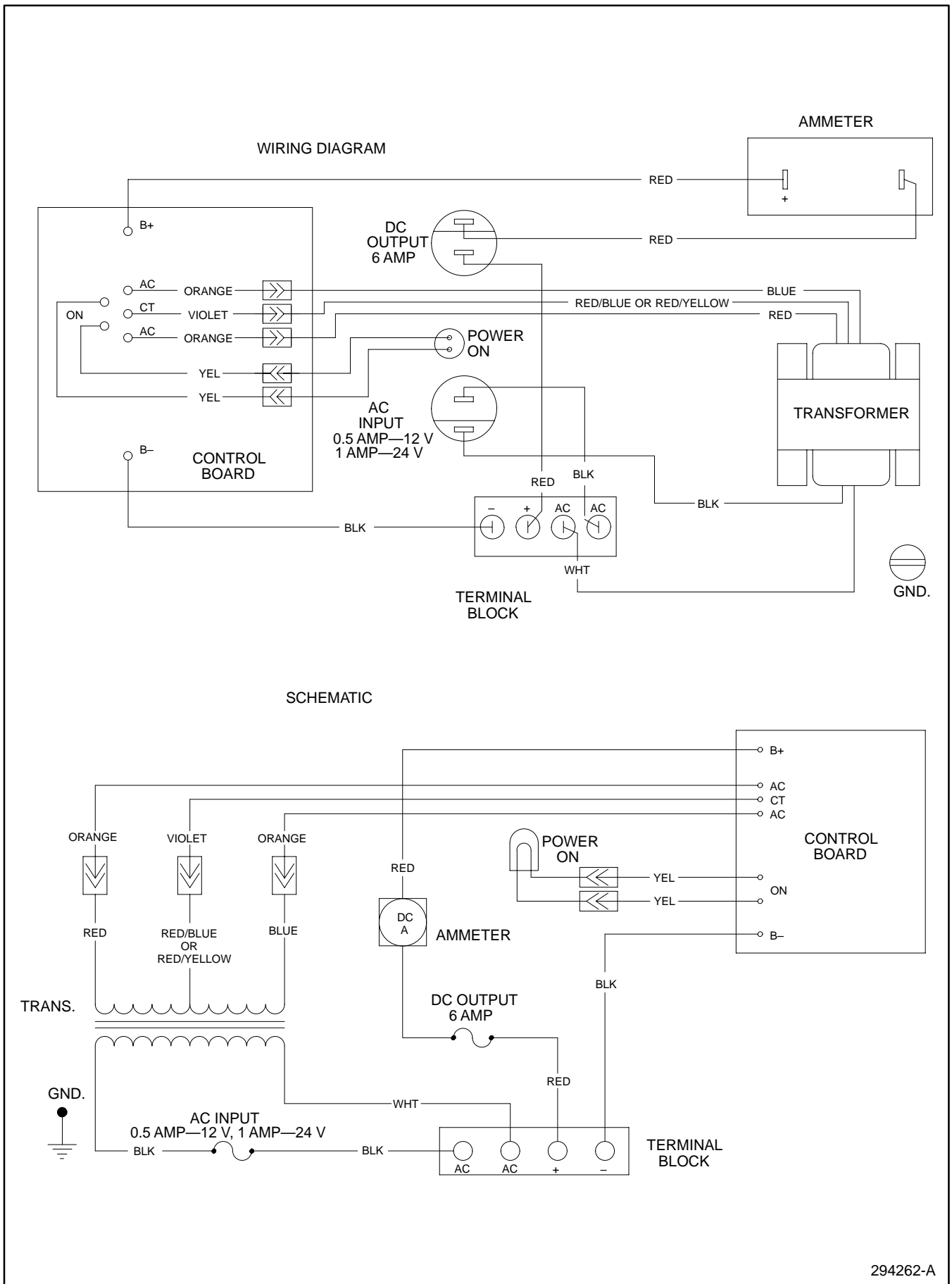
Figure 11. Wiring Diagram, Schematic—208-Volt Battery Charger
