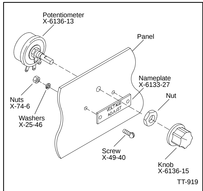
Figure 1. Potentiometer Installation
