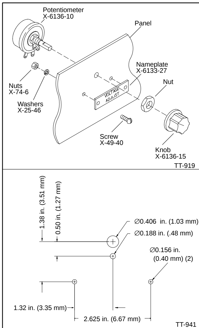
Figure 1. Potentiometer Installation
